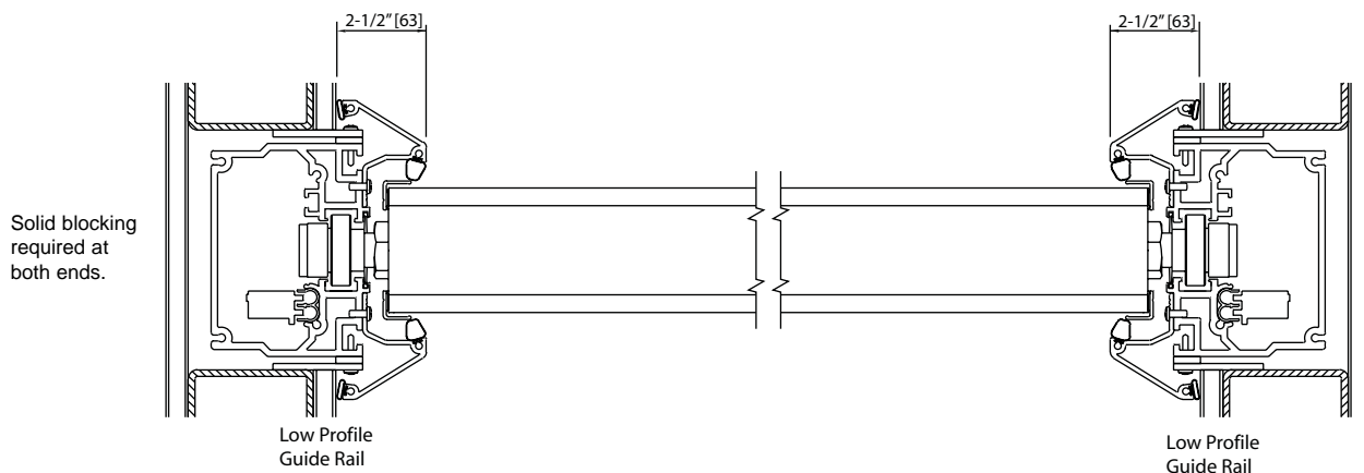
HORIZONTAL SECTION - Low Profile Mount
