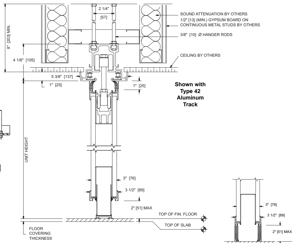
Optional: Bottom continuous contact (sweep) seals
