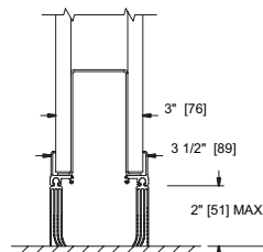
Optional: Bottom continuous contact (sweep) seals
